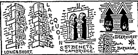
FIG. 30.—CELTO-SAXON DETAILS.
